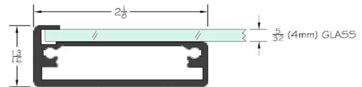
MONZA I CROSS SECTION
