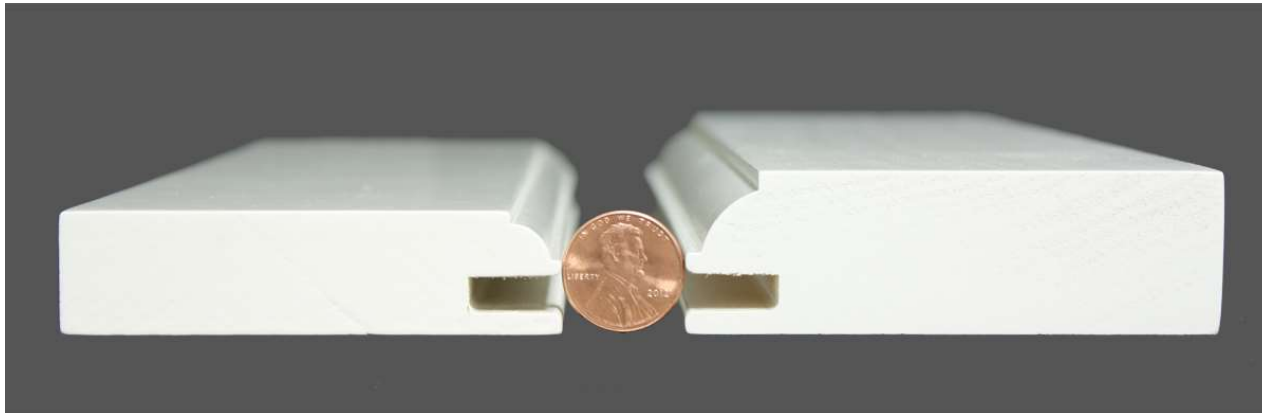
BEAD & FILLET ~ 3/4" DOOR THICKNESS
